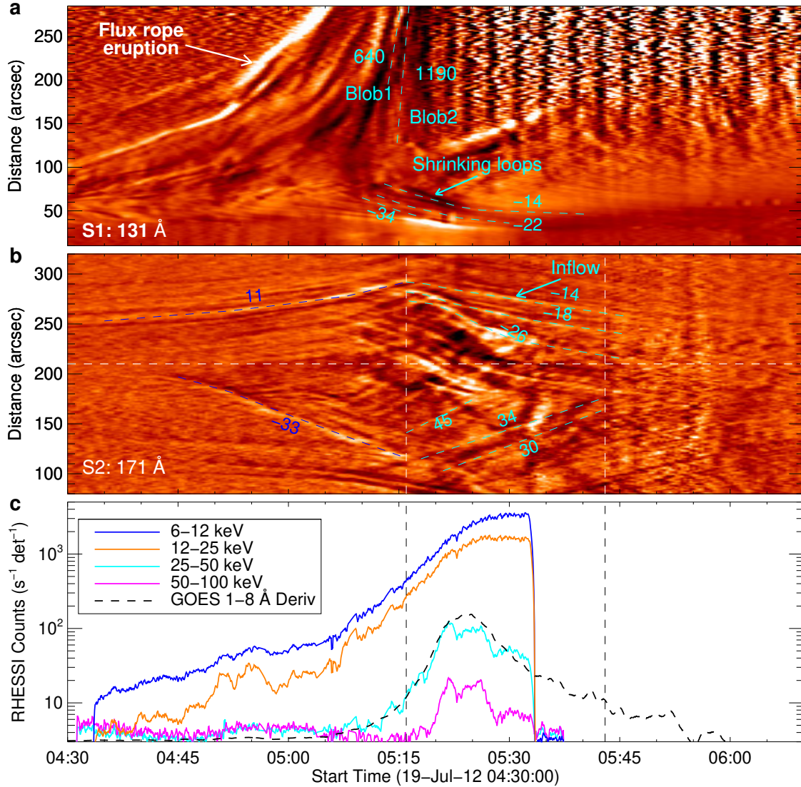
Figure 2. Temporal evolution of plasma inflows and outflows during the magnetic reconnection as observed in EUV by SDO/AIA. (a) Time-distance plot in AIA 131 Å along the current sheet (S1), showing the eruption of the flux rope and the bi-directional reconnection outflows. (b) Time-distance plot in AIA 171 Å along S2 (perpendicular to the current sheet), showing the separation (blue lines) and approach (cyan lines) of oppositely directed magnetic structures (the numbers denote the average speeds in units of km s -1 ). The horizontal white dashed line denotes the position of the current sheet. (c) Time profiles of the RHESSI X-ray emission in different energy bands and time derivative of GOES flux in 1-8 Å. The two vertical dashed lines indicate the flare impulsive phase.
