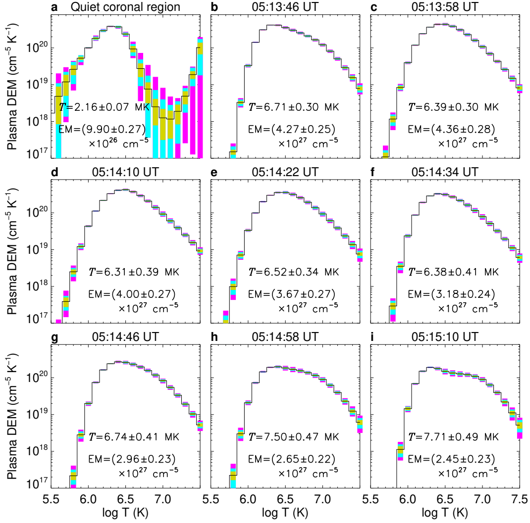
Figure S1. Panel (a): DEM of the quiet coronal region (R1 in Fig. 1g), Panels (b-i): DEM of the blob region (R2 in Fig. 1g) at eight selected times. The yellow, cyan and purple colors represent regions in which 50%, 80% and 95% of 100 Monte Carlo (MC) solutions are contained, respectively. The black line represents the best-fit DEM distribution. The total emission measure and the DEM-weighted temperatures are given in each panel. Three standard deviations ( 3\sigma ) of the 100 Monte Carlo simulations are regarded as the uncertainties.
