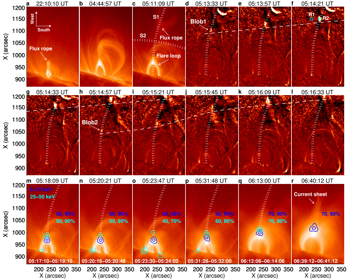
Figure 1. Snapshots of the eruption recorded by the 131 \text{ \AA} filter of SDO/AIA. West is rotated to the top and south to the right. Panel(a) shows the flux rope formed in an earlier confined C4.5 flare. Panels (b-r) show the eruption and evolution of the flux rope and the associated M7.7 flare. “S1” and “S2” in panel (c) indicate two slits placed along and perpendicular to the current sheet. Panels (d-l) are running ratio images, showing motions of two blob-like plasmoids. “R1” and “R2” in panel (f) indicate two subregions used for the DEM analysis. The arrow in panel (r) refers to the long current sheet. The contours overplotted in panels (m)-(r) show the RHESSI X-ray sources at 6-12 keV (blue) and 25-50 keV (cyan) reconstructed with the “clean” algorithm. The percentages define the contour levels.
